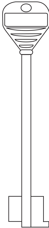
SK030 120 mm ø INT 3.5 ø EXT 6
