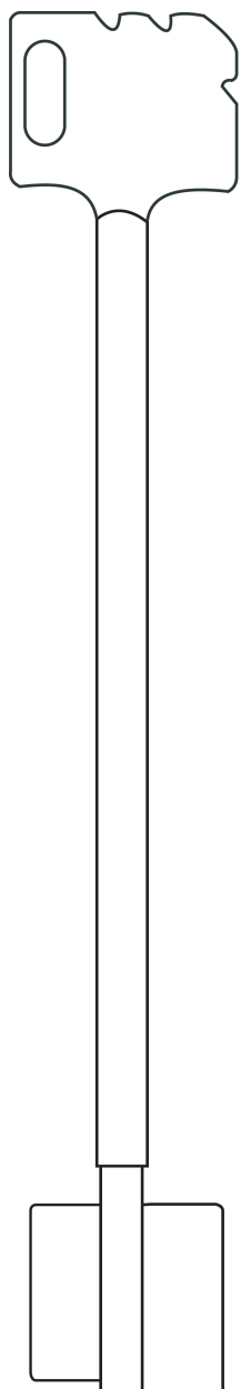
MAU1A 165 mm ø INT 3.5 ø EXT 6.8
