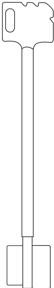
MAU3 146 mm ø INT 3.5 ø EXT 6.8
